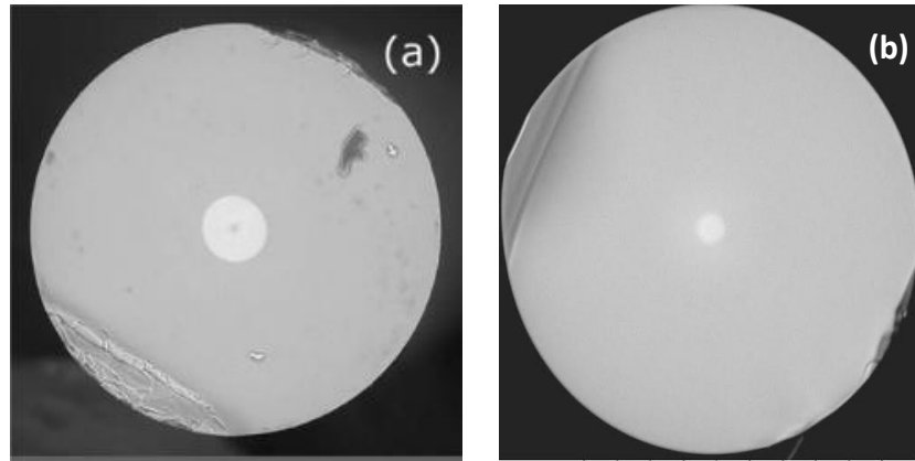
Figure 2. SEM of cross section of optical fibers core doped with (a) thallium, (b) germanium.
