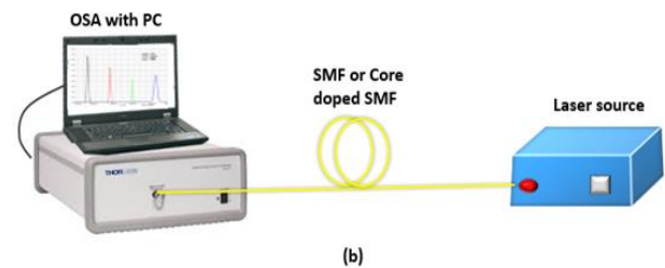
Figure 1. The optical fiber communication link, (a) photographic image, (b) schematic diagram.
