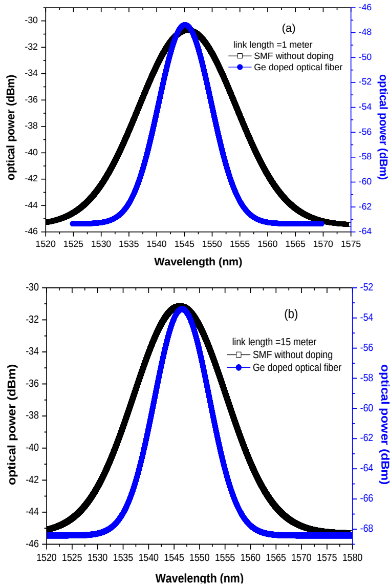
Figure 3. The optical spectra of SMF (without doping) and Ge-core doped core with link length (a) 1m, (b) 15m.
