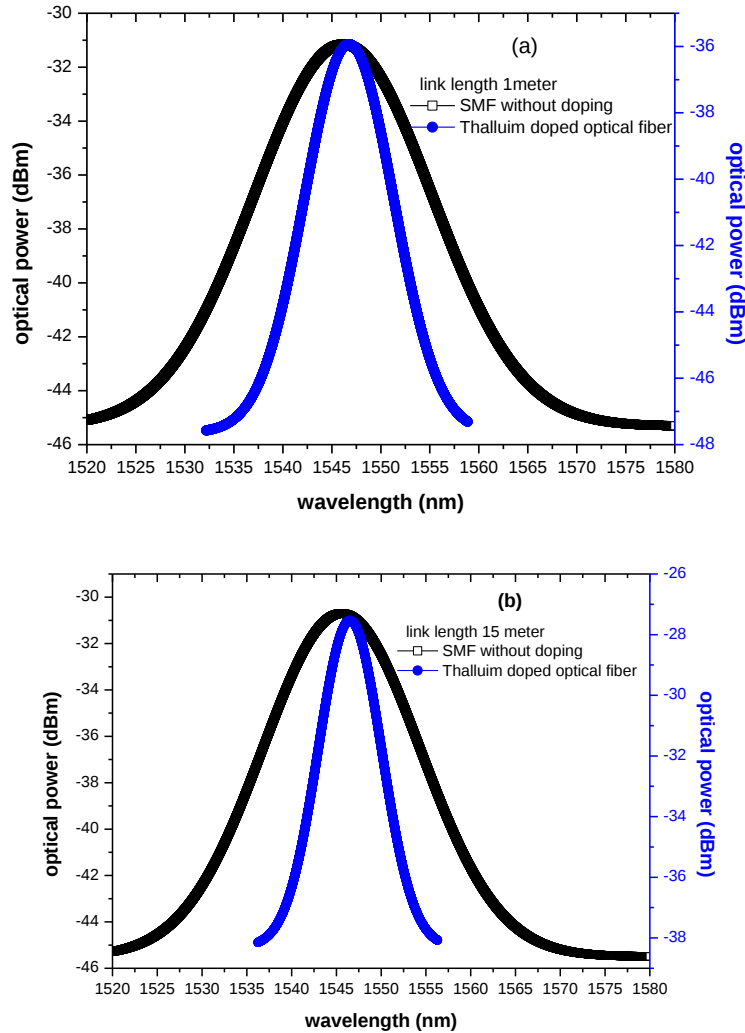
Figure 4. The optical spectra of SMF (without doping) and Tl-core doped core with link length (a) 1m, (b) 15m.
